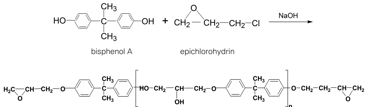
Scheme 2. Synthesis of bisphenol A type epoxy resin.
