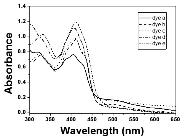
Figure 3. Absorption spectra of dye a–e in DMF.
