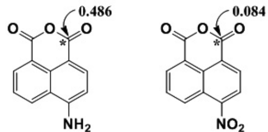
Figure 6. π-electron density of LUMO of (a) 4-amino-1,8-naphthalic anhydride and (b) 4-nitro-1,8-naphthalic anhydride.
