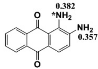
Figure 5. π-electron density of HOMO of 1,2-diaminoanthraquinone.
