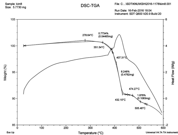
Figure 4. TGA analysis of dye a-e.
