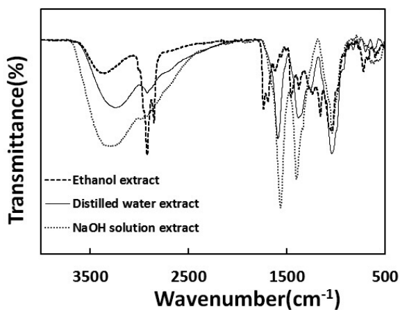
Figure 2. FT-IR spectra of Perilla Frutescens L. Britt extract.
