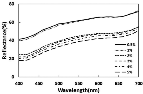
Figure 4. Reflectance curve of silk fabrics dyed with Perilla Frutescens L. Britt NaOH aqueous solution extracts(80°C, 60min).
