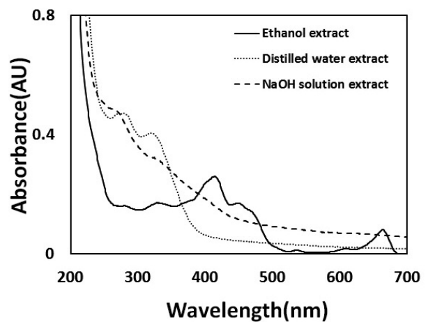
Figure 1. Ultraviolet-visible spectra of Perilla Frutescens L. Britt extracts.
