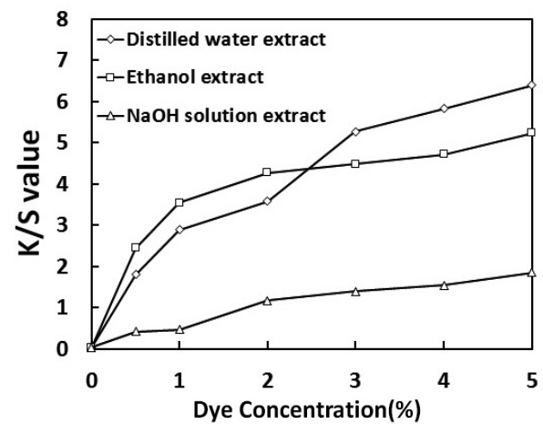
Figure 6. Effect of dye concentration on the dye uptake of silk fabrics dyed with Perilla Frutescens L. Britt extracts(80°C, 60min).
