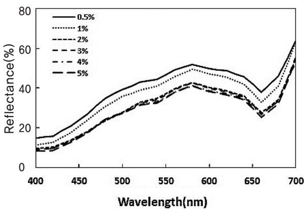
Figure 5. Reflectance curve of silk fabrics dyed with Perilla Frutescens L. Britt ethanol extracts(80°C, 60 min).
