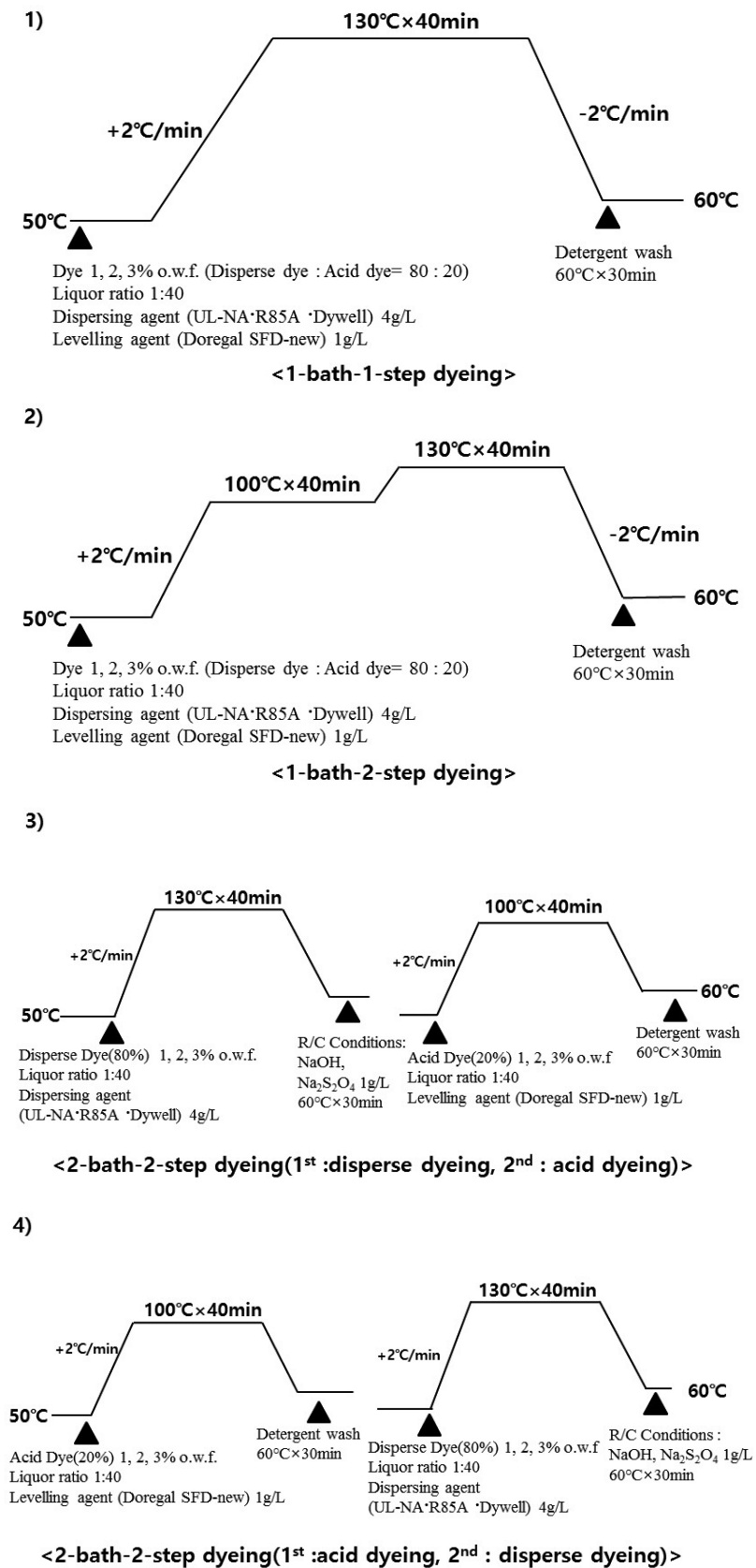
Figure 1. Dyeing profile.
