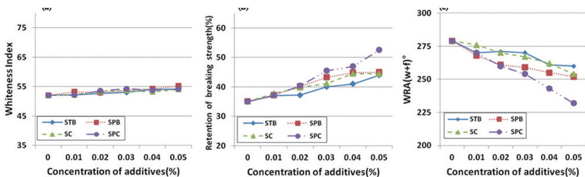
Figure 2. Effect of additives on (a) whiteness index, (b) retention of breaking strength, (c) wrinkle recovery angle of treated fabrics using one-bath method; glyoxal 5%owb, AS/glyoxal mole ratio=0.01.
