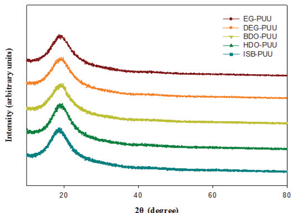
Figure 7. XRD curves of PUU films.
