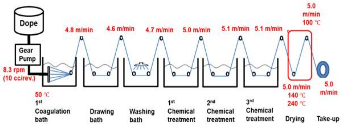
Figure 1. Schematic diagram for the preparation of alginate gelatin fiber.
