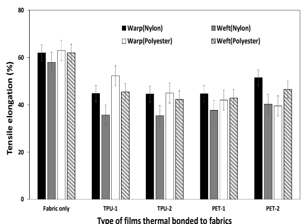
Figure 6. Tensile elongation of thermal bonded fabrics depending on various type of Warp of TPU and PET.
