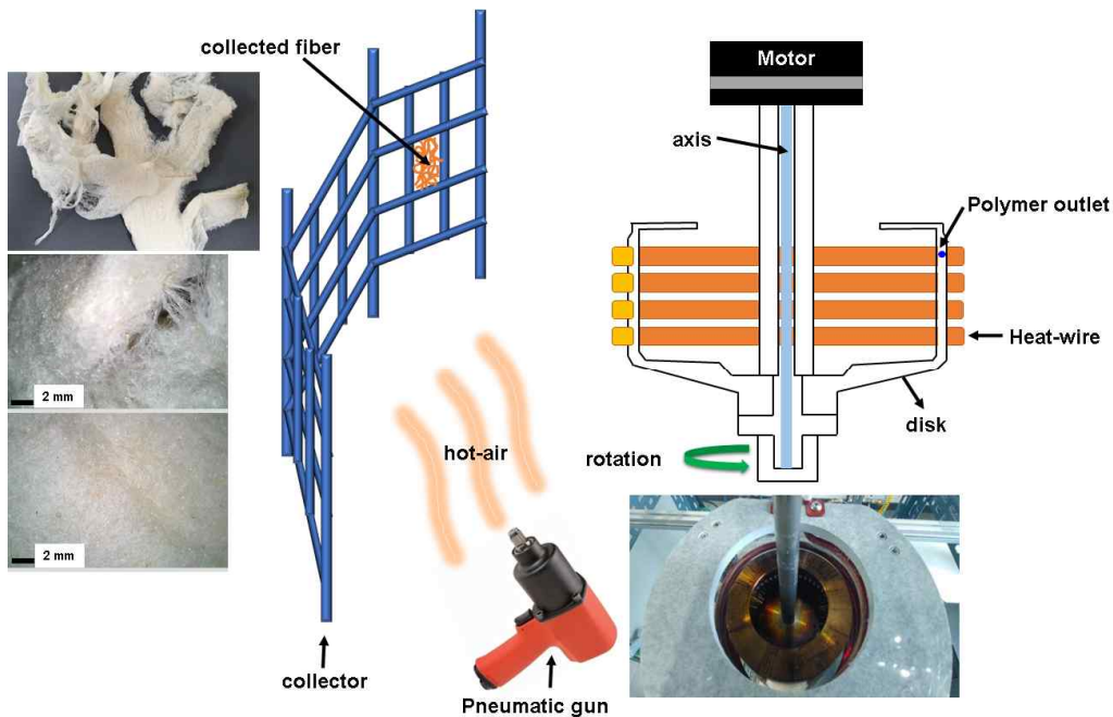
Figure 1. Schematic diagram of centrifugal melt spinning with hot-air.
