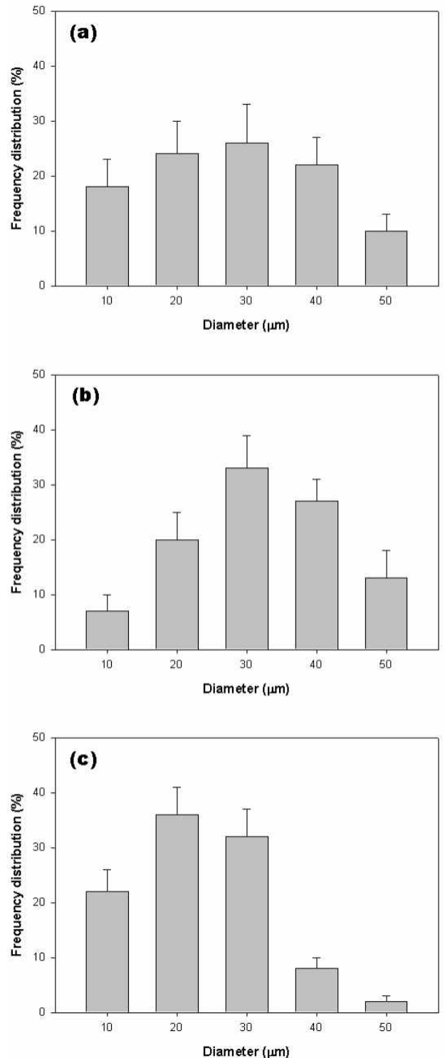
Figure 2. Diameter of fibers according to disk rotational velocity; (a) 6000 rpm, (b) 8000 rpm, and (c) 10000 rpm.
