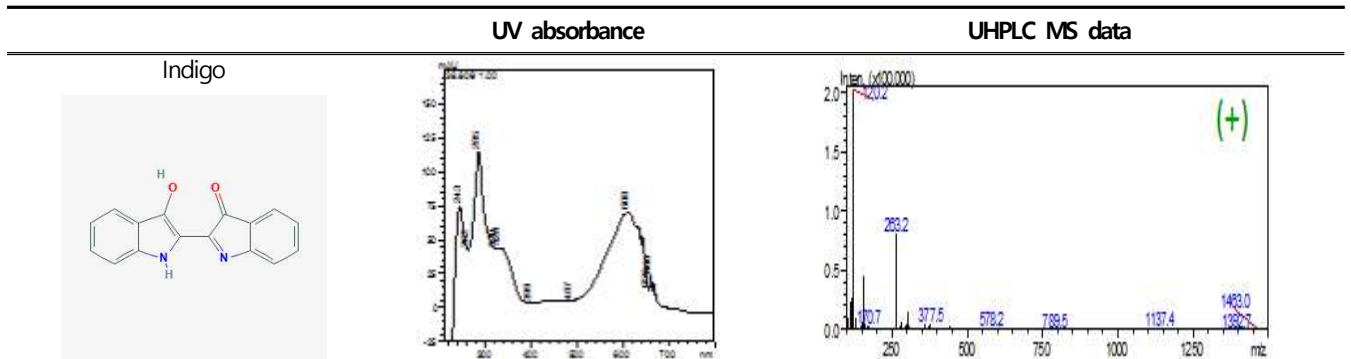
Figure 5. HPLC Chromatogram, DAD UV-Spectra and MS-data of insect natural dye.
