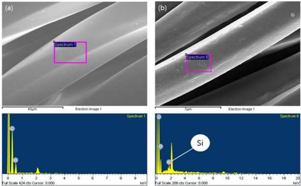
Figure 3. SEM-EDS analysis of (a) untreated PET and (b) treated with ODDMAC(130°C, 10min).
