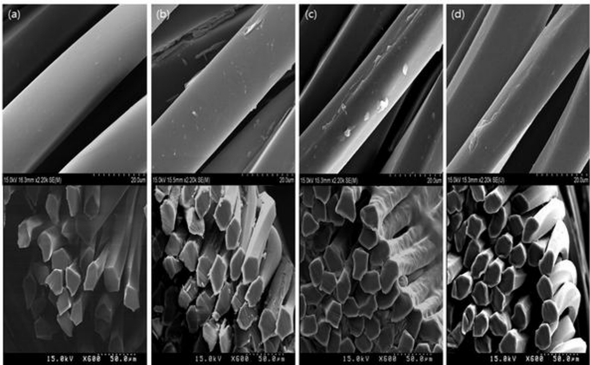
Figure 2. Surface and cross-sectional SEM image of (a) Untreated PET, treated PET with ODDMAC at 130°C for (b) 10min, (c) 10min and washed 25 cycles, (d) 10min and washed 50 cycles.
