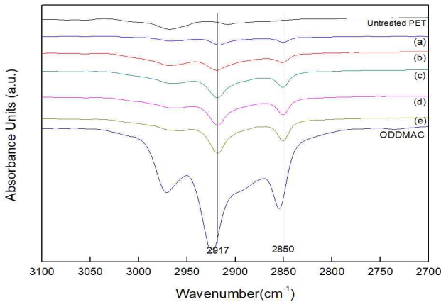
Figure 4. FTIR spectra of untreated PET and treated PET with the ODDMAC of (a) 5%, (b) 10%, (c) 15%, (d) 20%, (e) 25% at 130°C for 10min. The peaks at 2850 and 2917 \text{cm}^{-1} reflect the symmetric and asymmetric C-H stretching vibrations.
