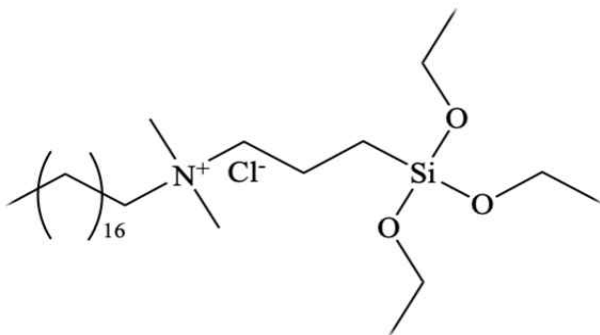
Figure 1. Octadecyldimethyl(3-triethoxy silylpropyl)ammonium chloride(ODDMAC) structure.
