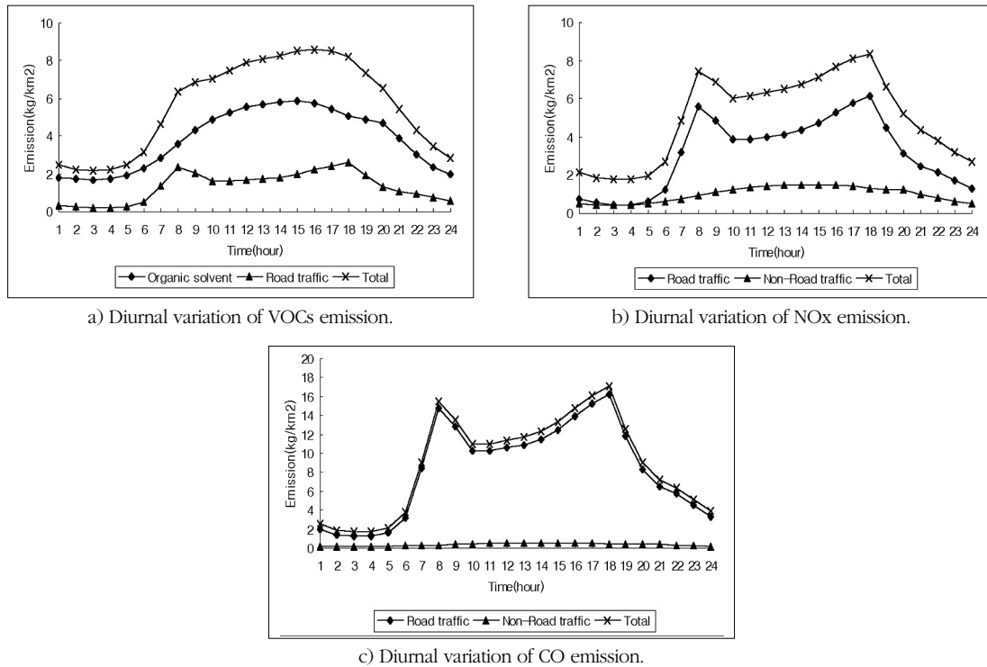
Figure 3. Diurnal variation of VOCs, NOx, CO emission
