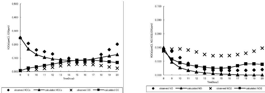
Figure 4. Comparisons of observed and calculated concentration
