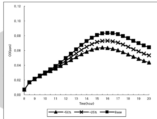
Figure 7. Diurnal variation of O 3 concentration by organic solvent reduction
