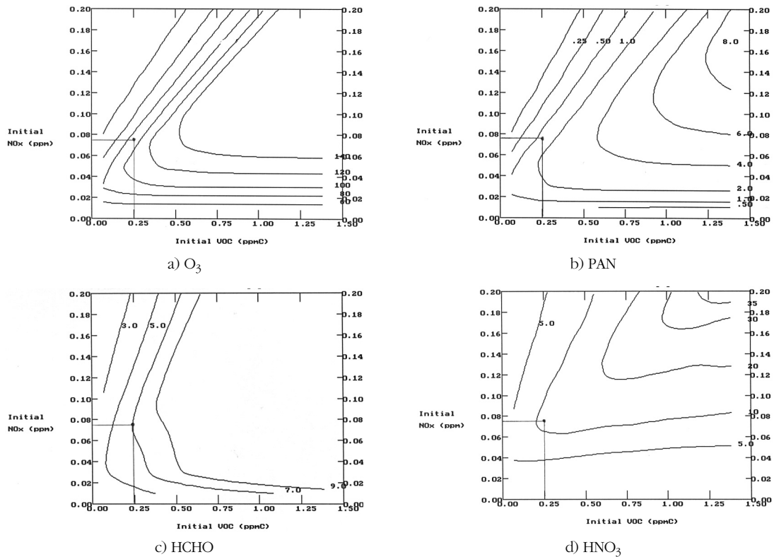
Figure 5. Ozone, PAN, HNO 3 , HCHO isopleth using OZIPR in Seoul
