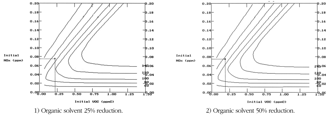
Figure 6. Ozone isopleth by organic solvent reduction
