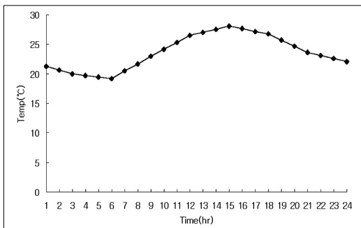
Figure 2. Diurnal variation of temperature in the summer of Seoul
