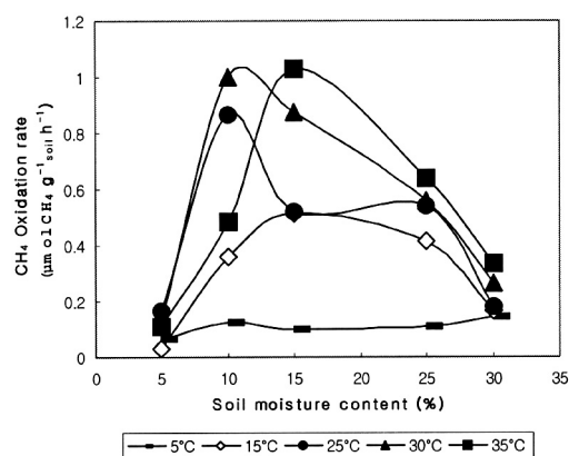
Figure 2. Methane oxidation rates as a function of soil moisture content and temperature
