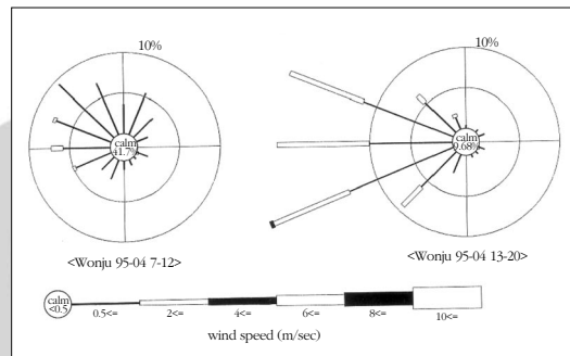
Fig. 6. The wind rose in Wonju at daytime (13-20 LST)
