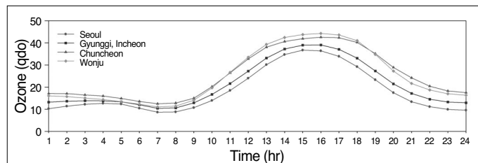
Fig. 4. Time series of daily average ozone concentration at Seoul, Gyeonggi · Incheon, Chuncheon and Wonju during April-September, 1995-2004
