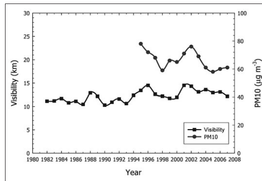
Fig. 3. Trend of visibility and the ambient PM10 concentration in Seoul
