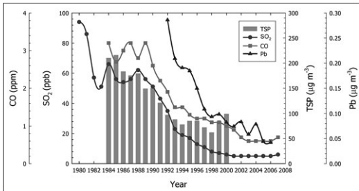
Fig. 1. Trend of the ambient concentrations of sulfur dioxide, carbon monoxide, TSP, and lead in Seoul
