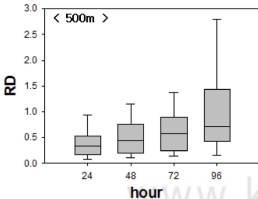
Figure 5. Percentile values(5, 25, 50, 75, 95 percentile) of relative distance(RD) between trajectories calculated using of MM5 and GDAS
