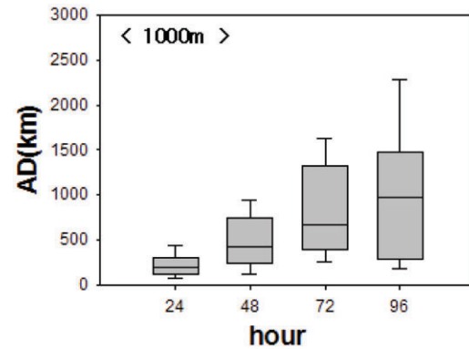
Figure 4. Percentile values(5, 25, 50, 75, 95 percentile) of absolute distance(AD) between trajectories calculated using of MM5 and GDAS
