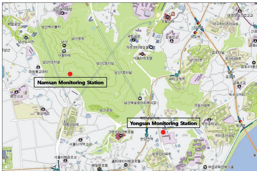
Figure 1. Location of Namsan and Yongsan-gu ambient air quality monitoring stations
