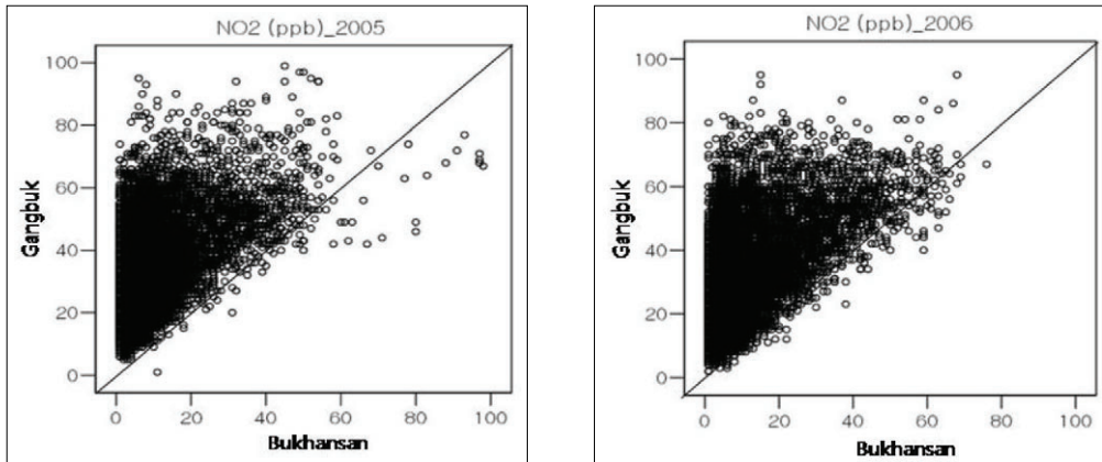
Figure 12. Correlation analysis of NO 2 in Bukhansan and Gangbuk
