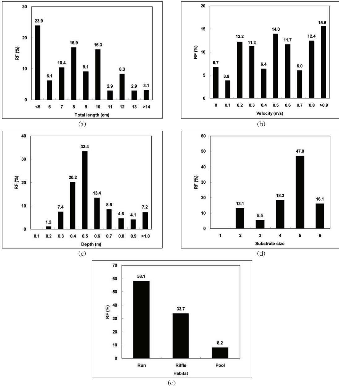
Figure 2. Relative frequency (RF) distribution on total length, velocity, depth, substrate size and habitat types in Zacco koreanus (n=781). Substrate size : 1(silt) : <0.062 mm, 2(sand) : 0.062~2.0 mm, 3(fine gravel) : 2.0~16.0 mm, 4(coarse gravel) : 16.0~64.0 mm, 5(cobbles) : 64.0~256.0 mm, 6(boulders) : >256.0 mm
