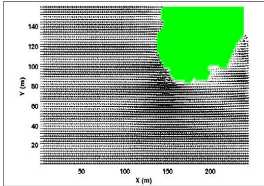
(a) W wind without the new building
