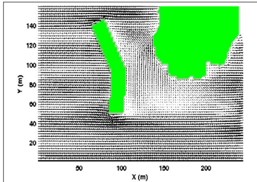
(c) W wind with the new building
