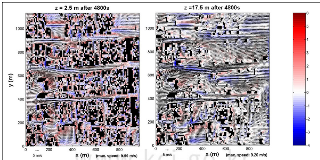
Fig. 1. Wind fields (shading: vertical velocity) at t=80\text{min} at two heights with surface heating observed by Terra on Apr. 17, 2004.
