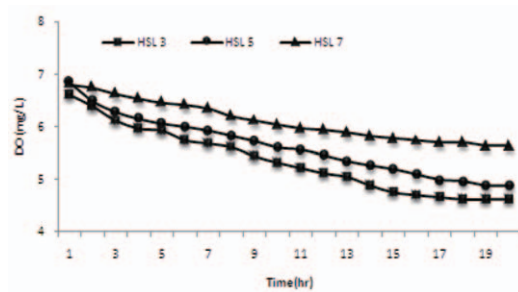
Figure 4. The change of dissolved oxygen (DO) concentration to estimate sediment oxygen demand(SOD)
