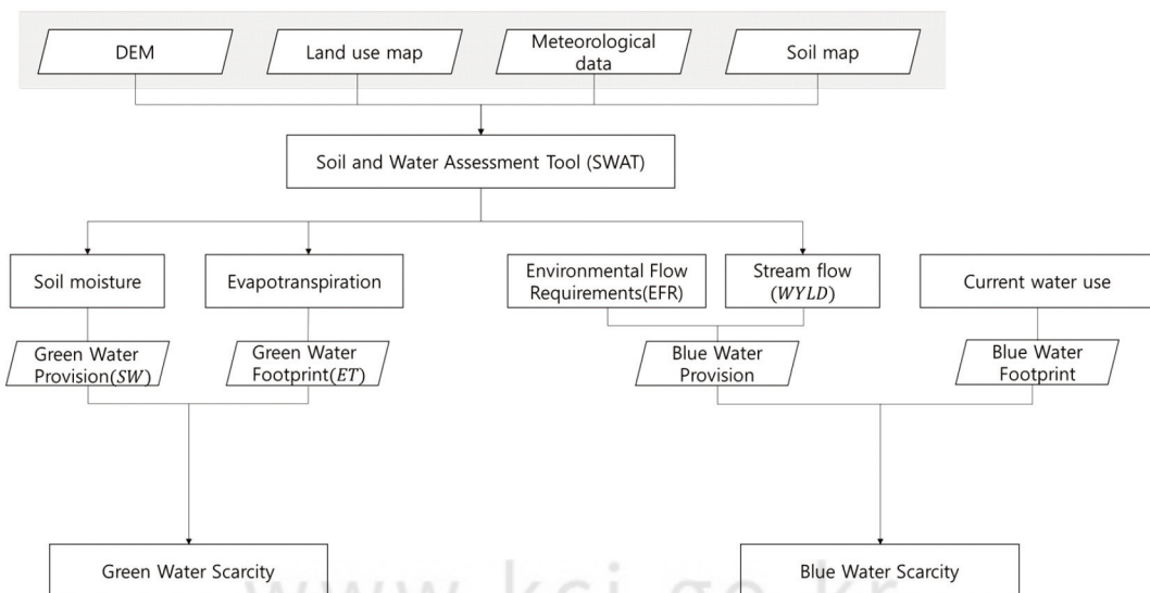
Figure 1. Study Flow.
