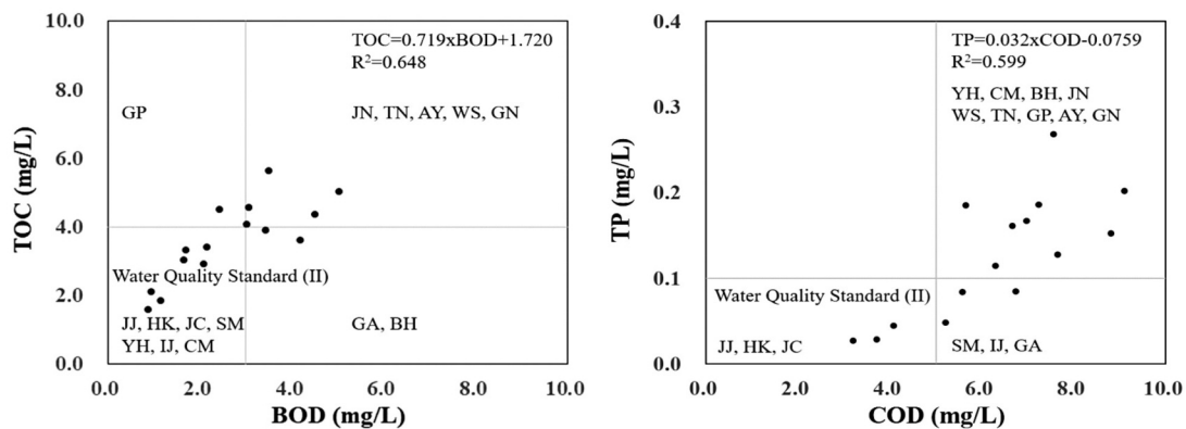
Figure 2. The relationship between BOD-TOC and COD-TP concentration in the Han River watershed tributaries.
