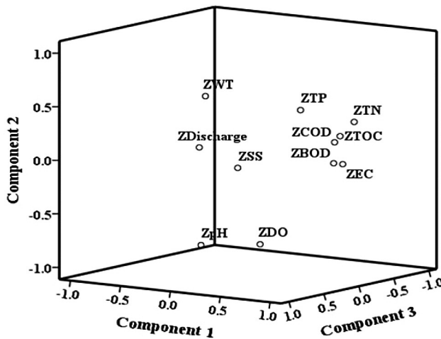
Figure 4. Component plot in rotated space.
