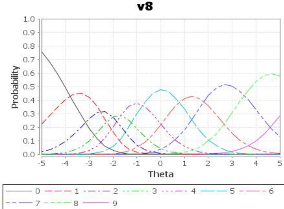
<Figure 2> Probability curves of K-SCCCS
