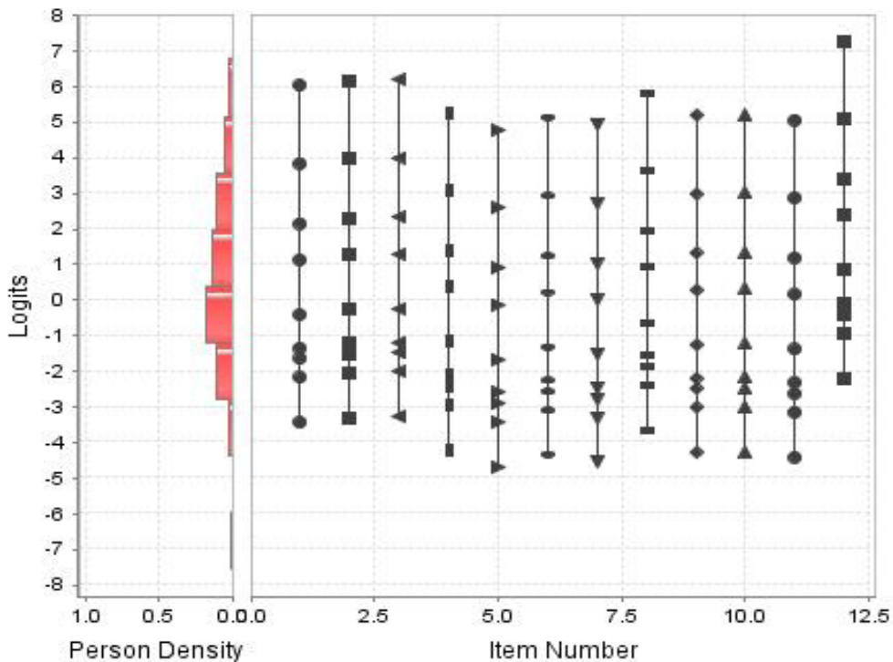
<Figure 1> Item person map of K-SCCCS
